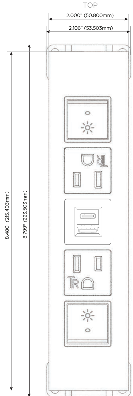
Shown with 2 Tamper Resistant ACs, and 1 USB-A & 1 USB-C Charging Port, and 2 Switched ACs (Rocker Switches).
