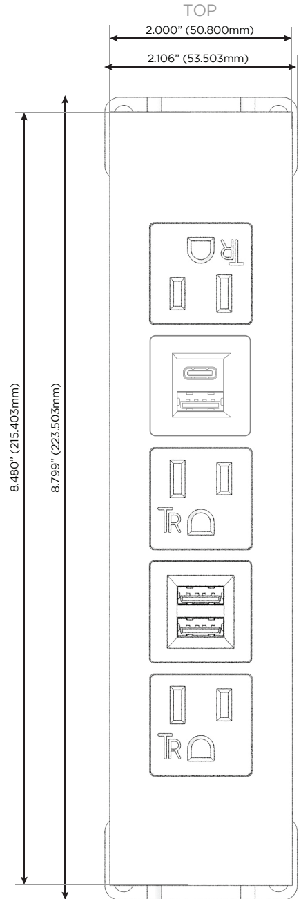
Shown with 3 Tamper Resistant ACs, 1 Double USB-A Charging Port, and 1 USB-A & 1 USB-C Charging Port.
