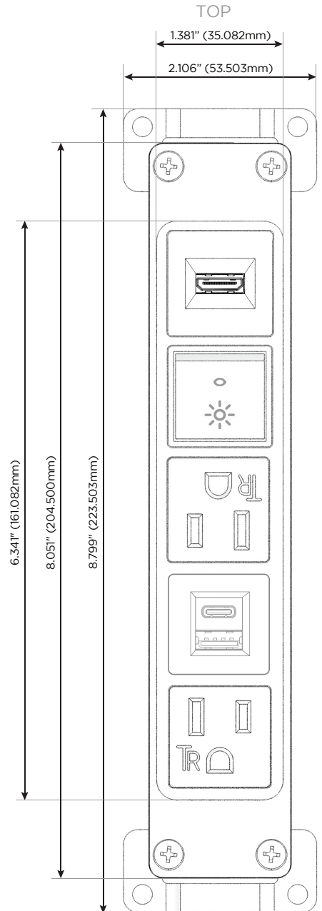
Shown with 2 Tamper Resistant ACs, 1 USB-A & 1 USB-C Charging Port, 1 HDMI Port, and 1 Switched AC (Rocker Switch).
