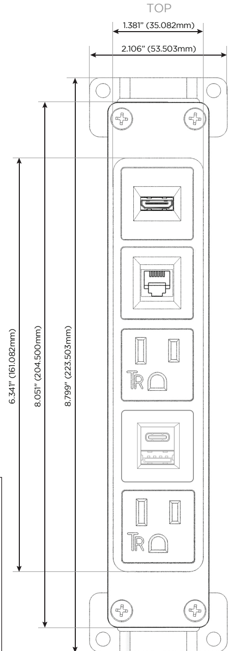
Shown with 2 Tamper Resistant ACs, 1 USB-A & 1 USB-C Charging Port, 1 RJ 12 Port, and 1 HDMI Port.
