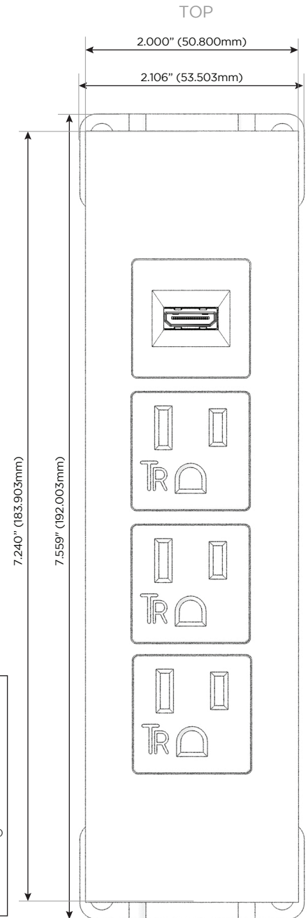
Shown with 3 Tamper Resistant ACs and 1 HDMI Port.
