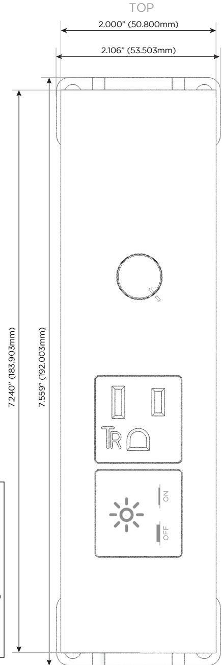
Shown with 1 Switched AC, 1 Tamper Resistant AC, and 1 AC Dimmer.
