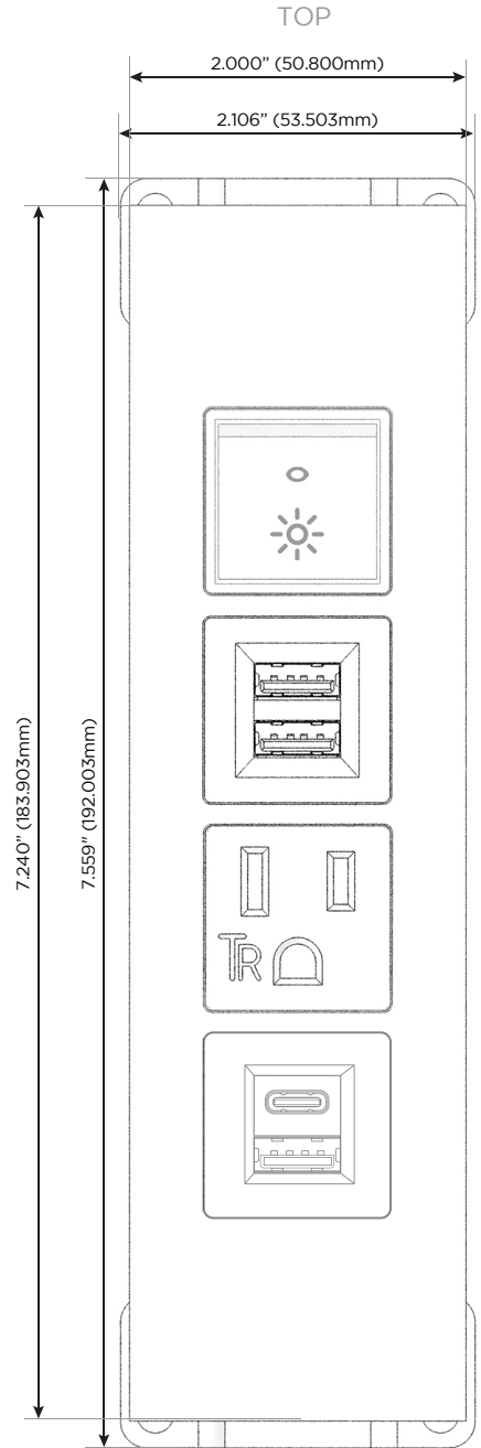
Shown with 1 USB-A & 1 USB-C Charging Port, 1 Tamper Resistant AC, 1 Double USB-A Charging Port, and 1 Switched AC (Rocker Switch).
