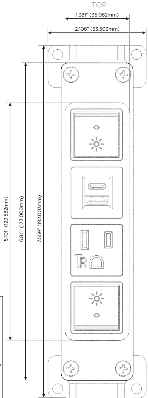
Shown with 2 Switched ACs (Rocker Switches), 1 Tamper Resistant AC, and 1 USB-A & 1 USB-C Charging Port.
