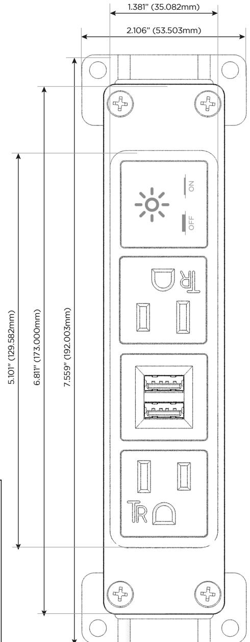
Shown with 2 Tamper Resistant ACs, 1 Double USB Charging Port, and 1 Switched AC.
