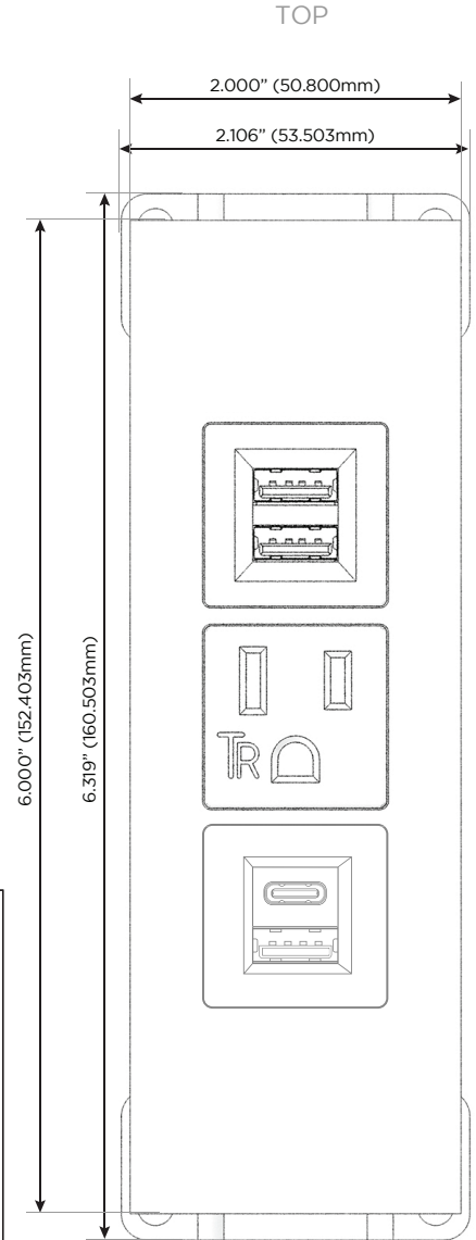
Shown with 1 USB-A & USB-C Charging Port, 1 Double USB-A Charging Port, and 1 Tamper Resistant AC.
