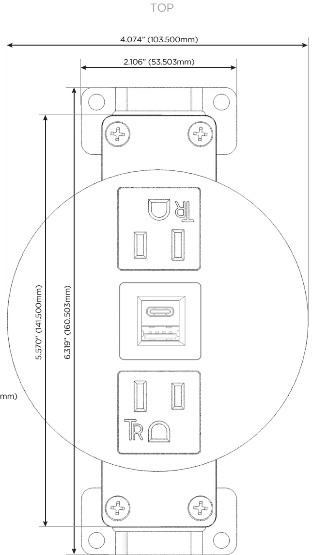
Shown with 2 Tamper Resistant ACs, and 1 USB-A & 1 USB-C Charging Port.
