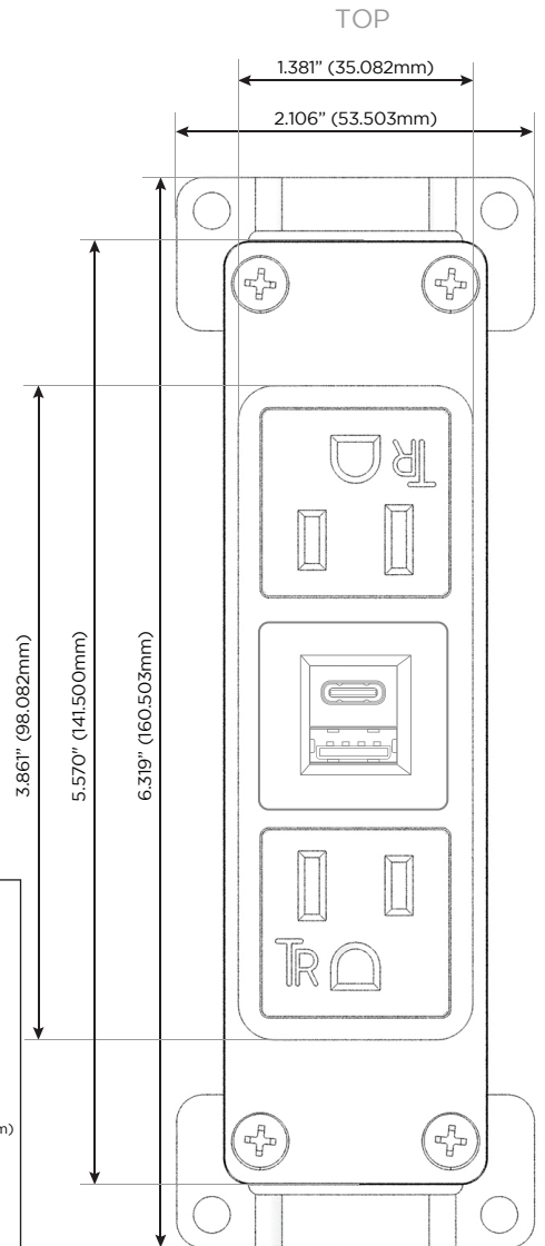
Shown with 2 Tamper Resistant ACs and 1 USB-A & 1 USB-C Charging Port.
