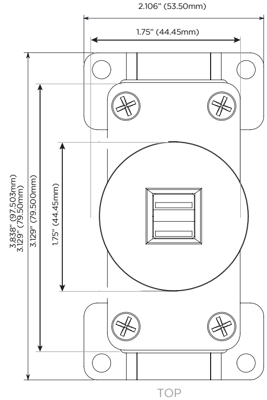
Shown with 1 Double USB-A Charging Port.
